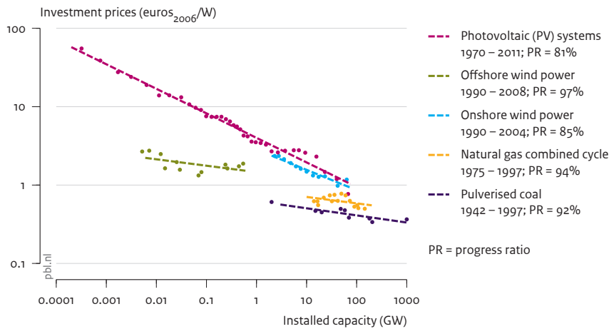
Figure 2.4 Learning curves of energy supply technologies
