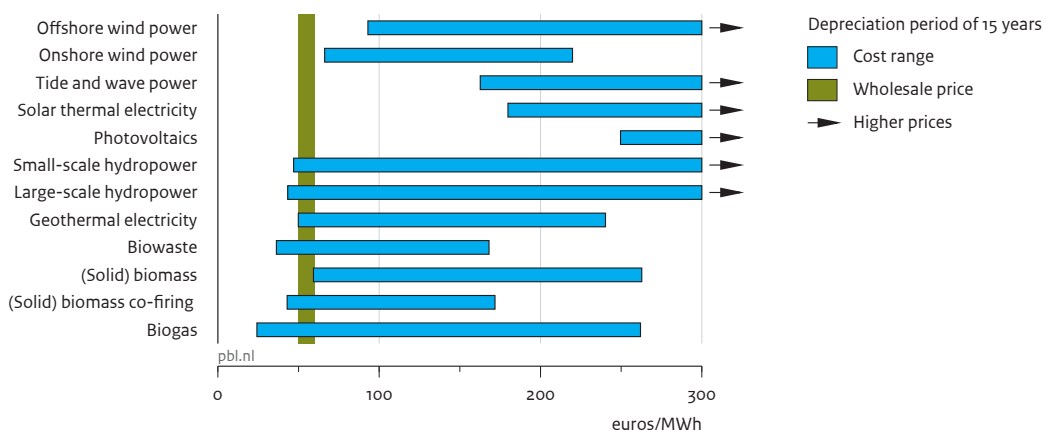
Figure 2.5 Costs of renewable electricity generation in the EU27, 2010
